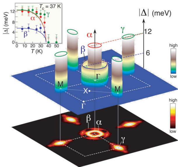
Fig. 4: (Colour on-line) Three-dimensional plot of the superconducting-gap size ( \Delta ) measured at 15K on the three observed FS sheets (shown at the bottom as an intensity plot) and their temperature evolutions (inset).
