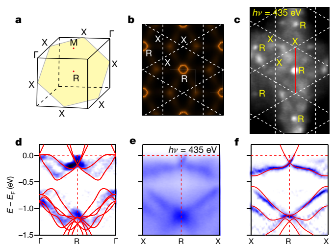
Fig. 2 | Fermi surfaces and band dispersions measured on the (111) surface. a , The hexagon in the three-dimensional BZ indicates the (111) plane that contains the R and X points. b , c , Calculated ( b ) and experimental ( c ) intensity plots at E_F showing the FSs in the (111) plane indicated in a . Dashed lines represent the intersecting lines of the (111) plane and the bulk BZ boundary. d , Curvature intensity plot of the ARPES data measured with varying h\nu from 325 eV to 580 eV, showing the band dispersions along R - \Gamma - R . The inner potential was set at 27 eV to fit the periodicity of band dispersions along R - \Gamma - R . e , f , Intensity ( e ) and curvature intensity ( f ) plots of the ARPES data along X - R - X . For comparison, we plot the calculated bands along R - \Gamma - R and X - R - X as red lines on top of the experimental data in d and f , respectively. The ARPES data in c , e and f were collected with h\nu = 435 \text{ eV} .
