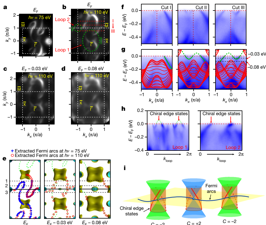
Fig. 4 | Surface Fermi arcs measured with VUV light on the (001) surface. a , ARPES intensity map at E_F measured with h\nu = 75 eV. b–d , ARPES intensity maps at E_F ( b ), E_F - 0.03 eV ( c ) and E_F - 0.08 eV ( d ), measured with h\nu = 110 eV. The momentum locations of loops 1 and 2 and cuts I, II and III are indicated in b , e . Surface Fermi arcs extracted from the ARPES intensity maps at E_F (left), E_F - 0.03 eV (middle) and E_F - 0.08 eV (right), showing the connection between the (001) surface projections of the bulk FSs at \bar{\Gamma} and \bar{M} . The dashed lines indicate the momentum locations of cuts I, II and III. f , ARPES intensity plots showing the band dispersions along cuts I, II and III. For comparison, we plot the projections of the calculated bulk bands as red lines on top of the experimental data in g . Solid and dashed green lines in g are guides for the eye for the surface state bands. h , ARPES intensity plots showing the band dispersions on loops 1 and 2. i , Schematic showing chiral edge states on the loops that encircle the surface projections of bulk nodes with non-zero Chern numbers C = \pm 2 and surface Fermi arcs connecting the surface projections of bulk nodes with opposite chiralities.
